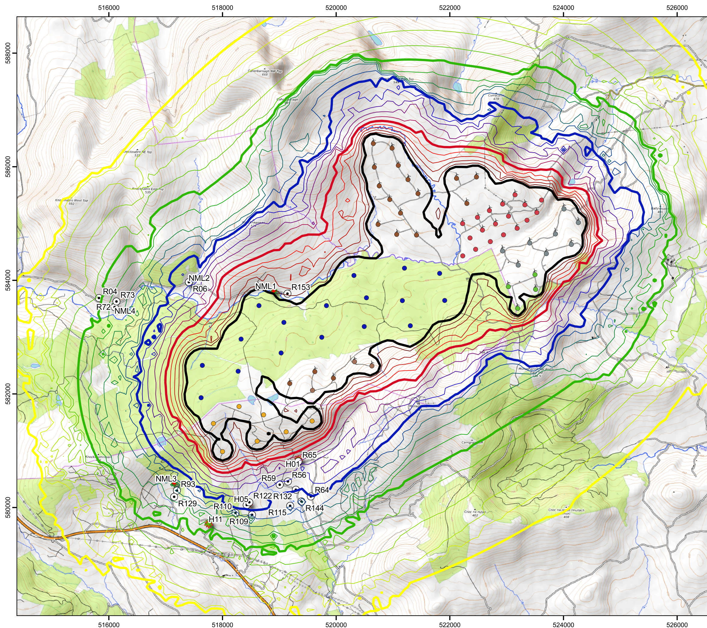
Figure 13-2 Predicted Operational Noise Levels at Rated Power - Cumulative
